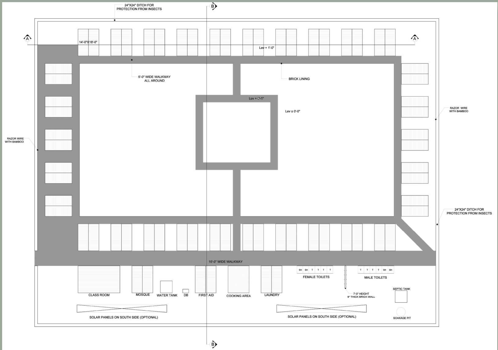
FLOOD RELIEF TENT VILLAGE - CONCEPT LAYOUT PLAN
